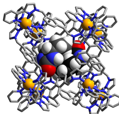
Figure 6. Structure of the complex \text{H}\cdot(\textbf{9})_2 with the host cage H in wireframe but the pair of guests 9 shown space-filling.
