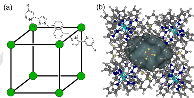
Figure 1. The host cages [Co_8L_{12}]^{16+} , abbreviated as H ( R = H ; soluble in MeCN) and H^w ( R = CH_2OH ; soluble in water). (a) A sketch emphasising the cubic array of Co(II) ions and the disposition of a bridging ligand; (b) a view showing the cavity space (volume 409\text{ Å}^3 ).
