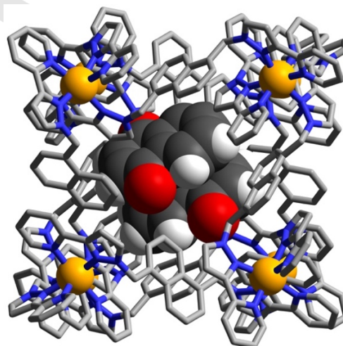
Figure 8. Structure of the complex \text{H}\cdot(\text{12})_2 with the host cage H in wireframe but the stacked pair of guests 12 shown space-filling.
