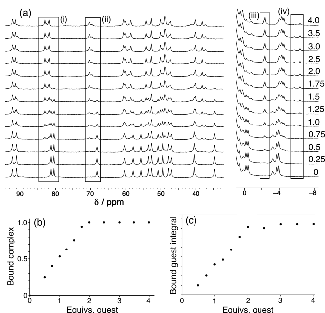
Figure 12. An NMR titration performed by addition of up to four equivalents of guest 4 to the \text{Co}_8 cage \text{H}^{\text{w}} (0.15 mM, \text{D}_2\text{O} , 298K). (a) Stacked plot showing evolution of the spectra as guest is added (number of equivalents of added guest is indicated). Boxes (i) and (ii) illustrate how the signals for empty cage (bottom spectrum) are replaced by new signals for bound cage (top spectrum): integration of these allows the fraction of cage occupied by guest to be determined in each spectrum. Boxes (iii) and (iv) illustrate the grow-in of signals for the bound guest in the paramagnetic cavity: integration of these allows a separate measurement of the fraction of cage occupied by guest during the titration. (b) Graph of fraction of complex containing guest (from 0 to 1) based on integration of free / bound cage signals at 68 – 70 ppm [box (ii) in part (a)]. (c) Graph of magnitude of integral for bound guest signal at –2.3 ppm [box (iii) in part (a)]. Both graphs (b) and (c) confirm strong binding of two guests under these conditions, see main text.
