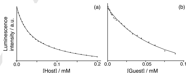
Figure 10. Luminescence titrations used to determine cage/guest binding constants in aqueous solution. (a) A solution of 10 \mu\text{M} of fluorescent guest 6 quenched by addition of increasing portions of the \text{Co}_5 cage \text{H}^\bullet (in this titration the normal roles of 'host' and 'guest' have been reversed for spectroscopic convenience). (b) A solution of 5 \mu\text{M} of fluorescent \text{Cd}_5 cage \text{H}^\bullet\cdot\text{Cd} , quenched on uptake of added guest 4 . In both cases good fits to a 1:1 binding model were obtained; see main text.
